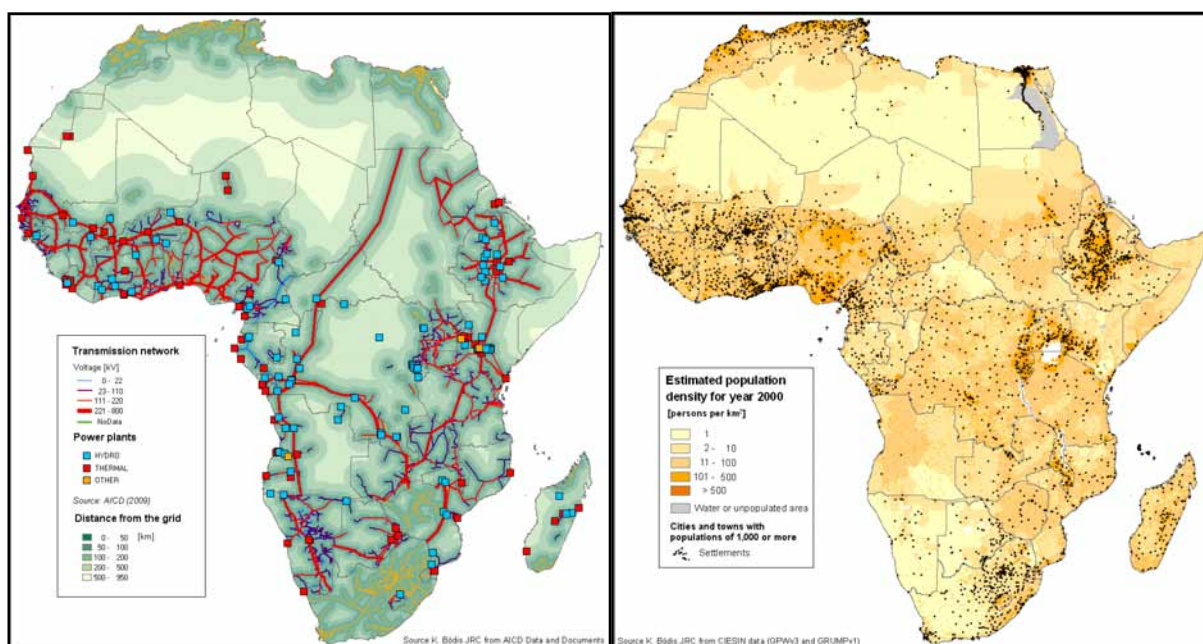
Figure 1.4 The geographical deployment and voltage capacity of electricity grid in African continent (yellow lines mean transmission/distribution grid existing but no data on capacity are available) and power plants in Sub-Saharan countries (left) and population density estimated in year 2000 in the African continent (right).
